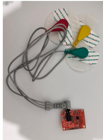
GAMBAR 2 Sensor AD8232
