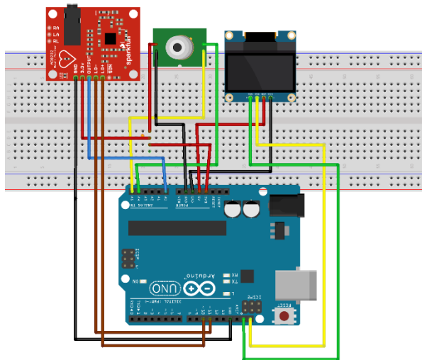
GAMBAR 5 Perancangan Hardware
